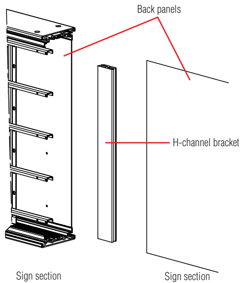
Figure 10: H-channel bracket preparation
