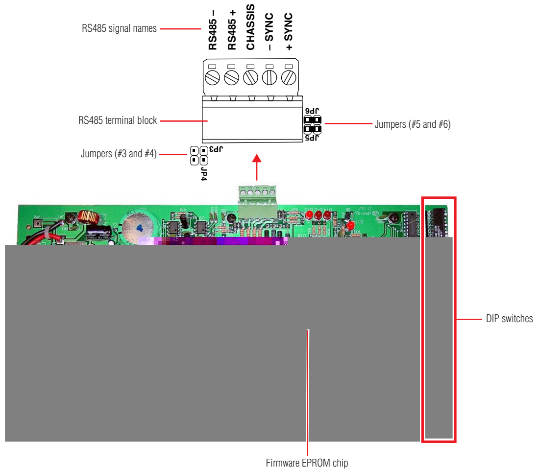
Figure 11: Controller board
