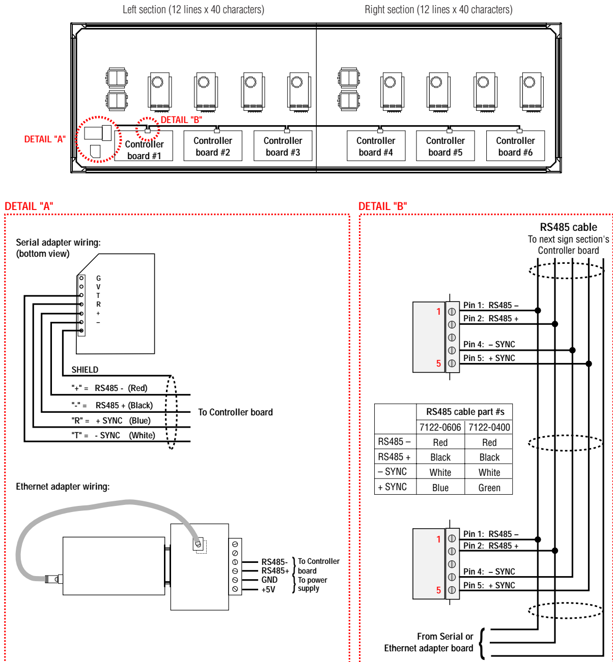
Figure 16: Multi-section sign network wiring
