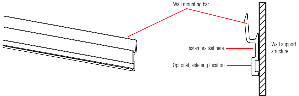
Figure 8: Wall mounting bar attachment
