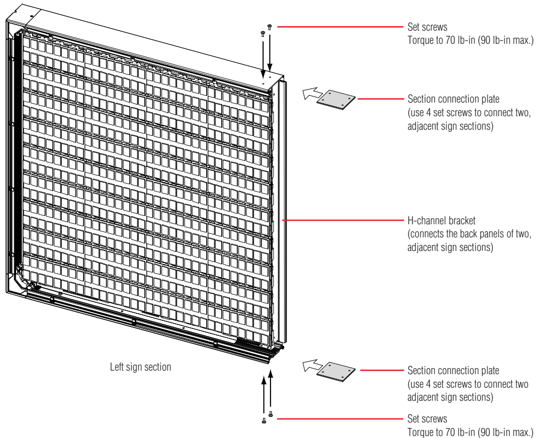
Figure 7: Section connection plate attachment
